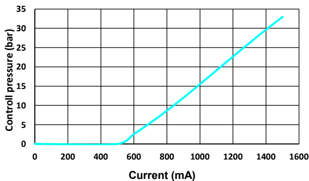
P-I CURVE (12V_4,72 \Omega )
