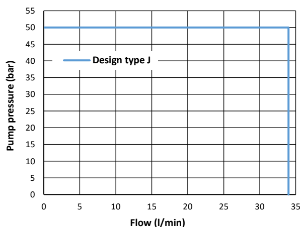
Switching limit for port assignment type J
