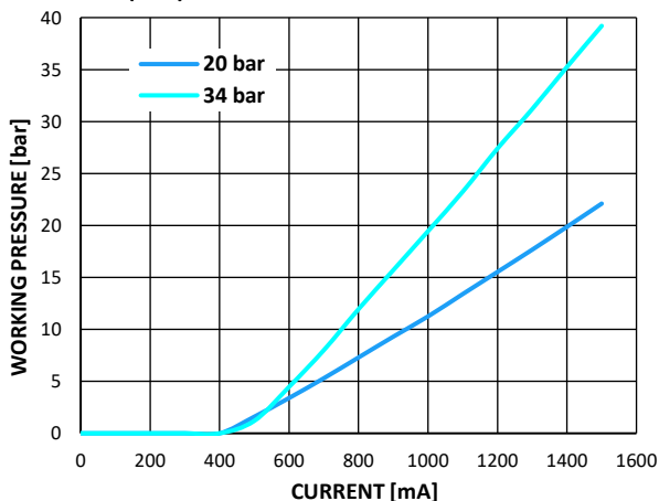
P-I CURVE (12V)
