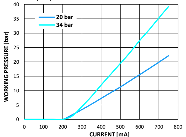
P-I CURVE (24V)
