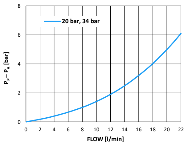
PRESSURE DROP PUMP TO CONTROL PORT (P→A)
