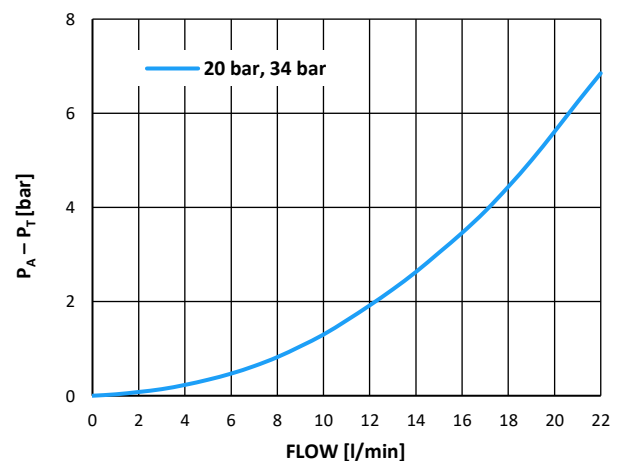
PRESSURE DROP CONTROL PORT TO TANK (A→T)
